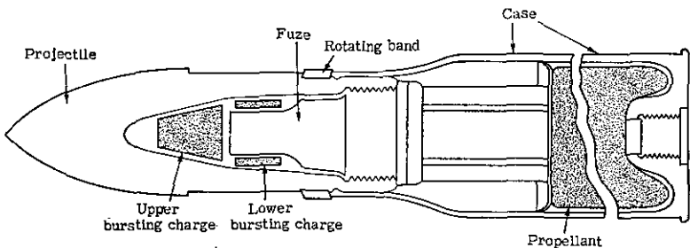
Figure 130.—Cross section of Model 94 (1934) armor-piercing shell.
