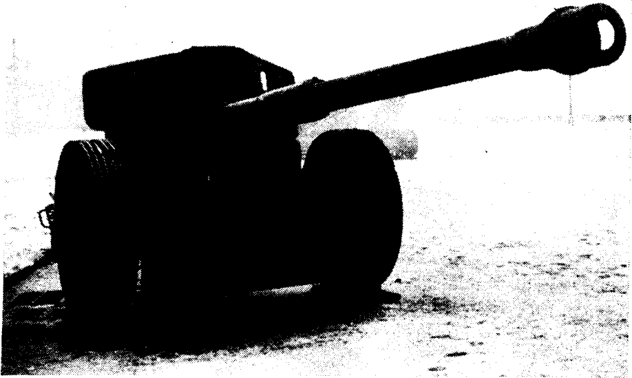
Figure 30.—Front view of the 88-mm antitank gun (8.8. cm Pak 43).
